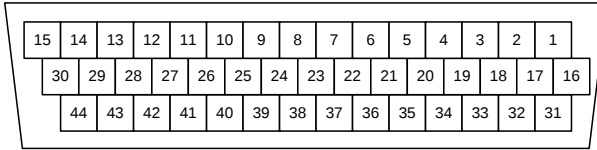
CN1 plug pin layout
