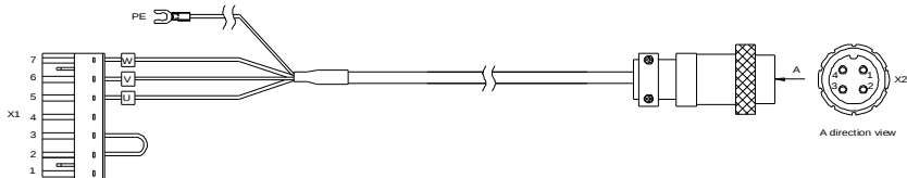
Wiring relation
